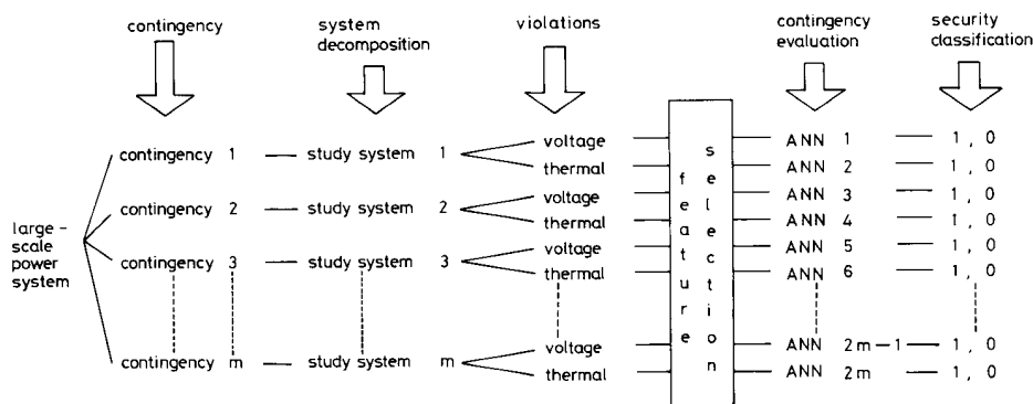
Fig. 1 Proposed NN approach to SSA
